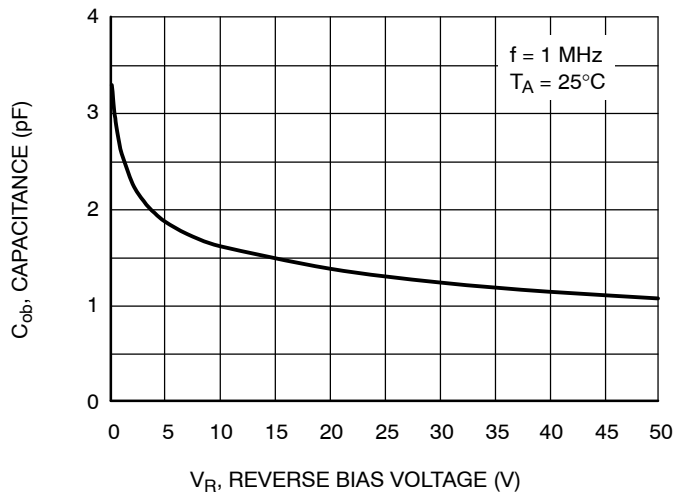
Figure 35. Output Capacitance
