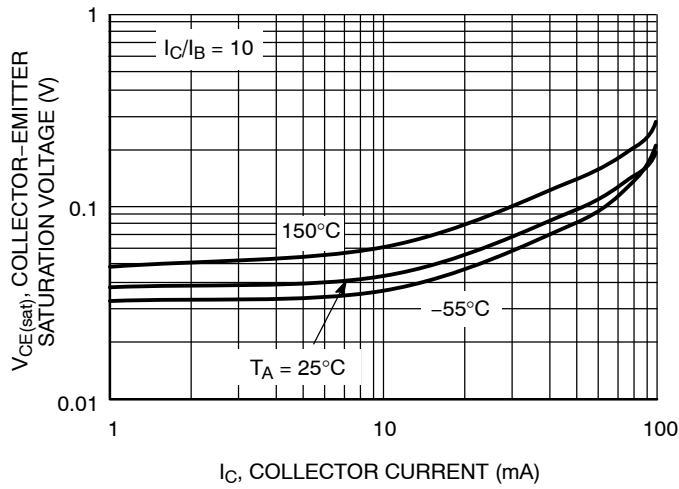
Figure 33. V_{CE(sat)} versus I_C
