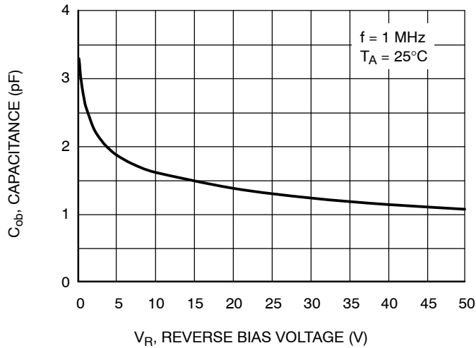
Figure 35. Output Capacitance
