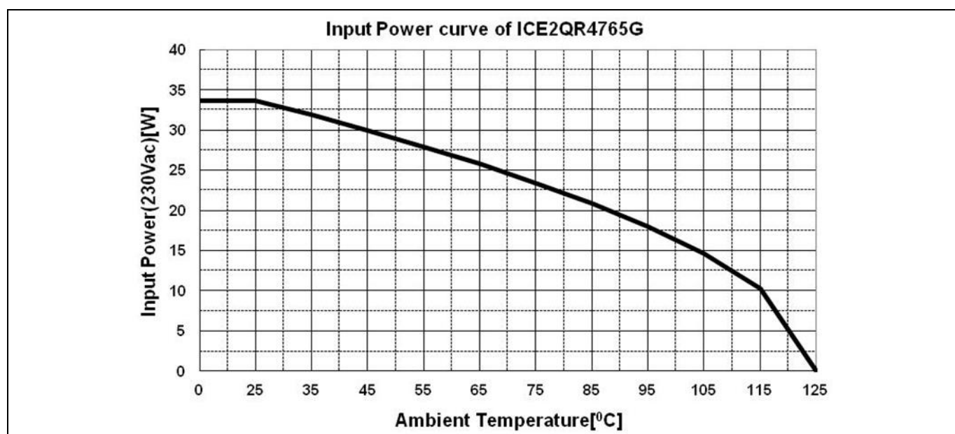
Figure 14 Input power curve V_{in}=230\text{ V}_{AC} ; P_{in}=f(T_a)
