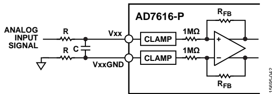
Figure 42. Input Resistance Matching on the Analog Input
