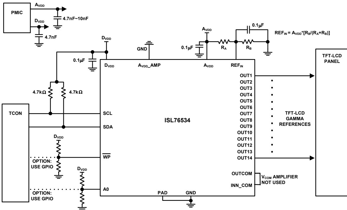
FIGURE 31. TFT-LCD GAMMA REFERENCE GENERATOR: VCOM AMPLIFIER DISABLED
