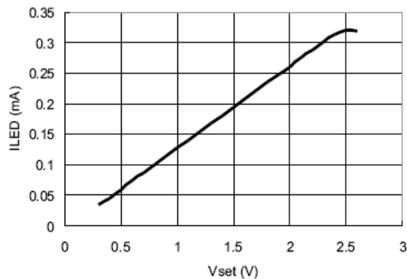
11. I_{LED} VS V_{SET} ( V_{IN}=16\text{V} , 3 LEDs, 47\mu\text{H} , R_s=0.15\Omega )
