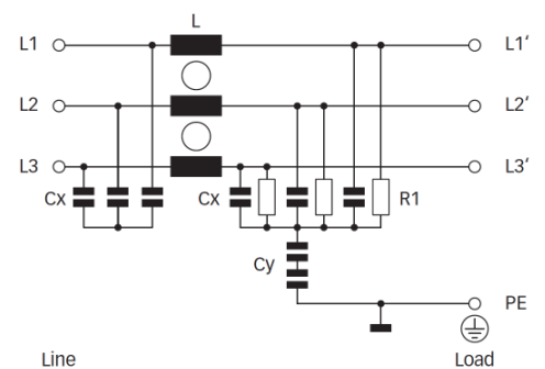
Typical electrical schematic
