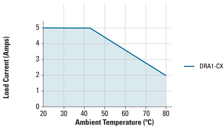
DRA1-CX Derating Curve
