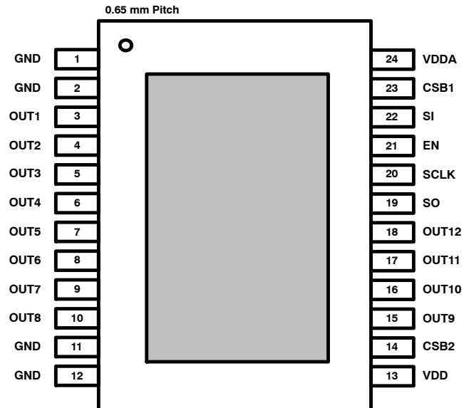
Figure 2. NCV7751 Pinout
