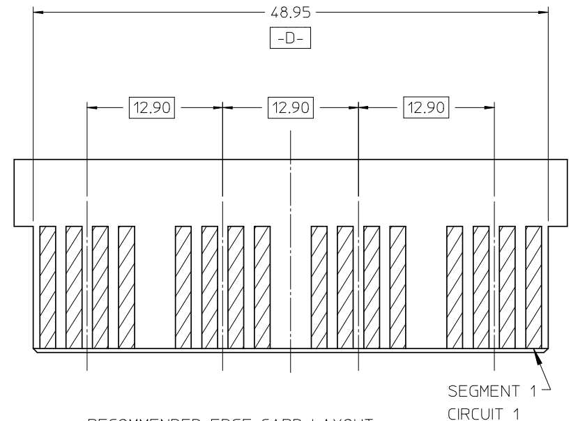
RECOMMENDED EDGE CARD LAYOUT TOLERANCE: \pm 0.05
