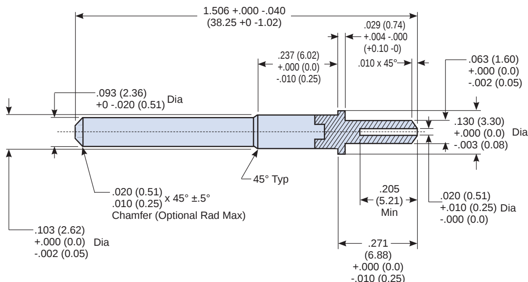
Dimensions and Configuration for Size 16 Contacts
