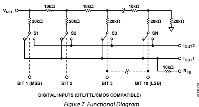
Figure 7. Functional Diagram
