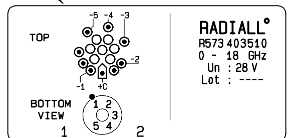
MARKING TOP VIEW (TERMINALS)
