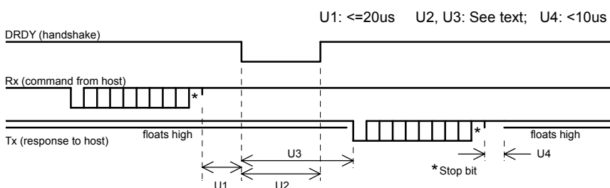
Figure 3-4 UART Timing
