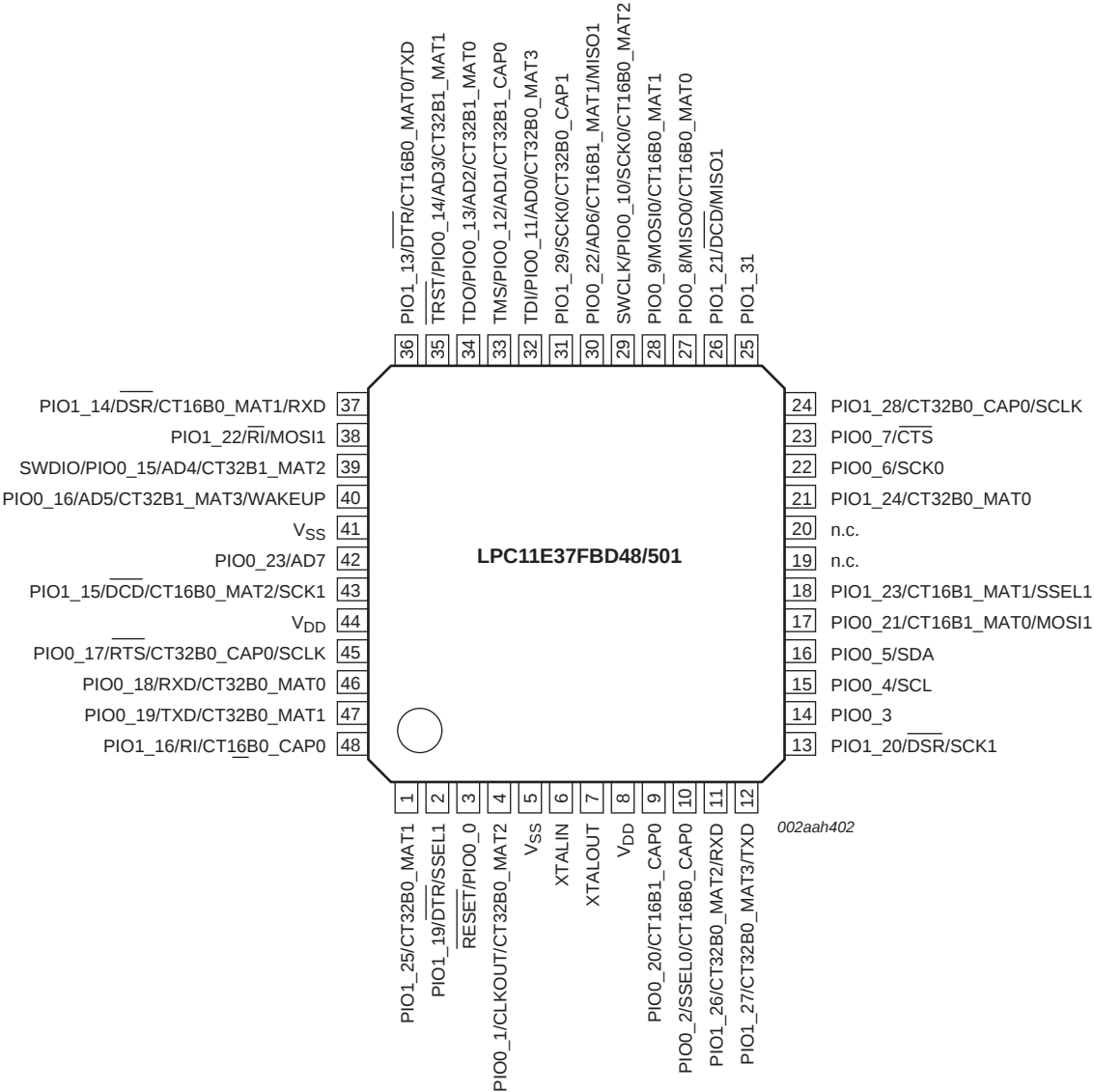
Fig 4. Pin configuration (LQFP48)
