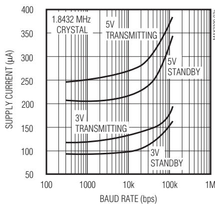
SUPPLY CURRENT vs. BAUD RATE
