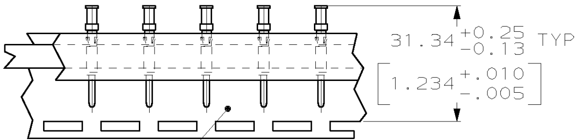
MYLAR TAPE TAPE MTG DETAIL \triangle 4 193844-2 ONLY
