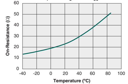
Typical On-Resistance vs. Temperature ( I_F=5\text{mA} , I_L=100\text{mA}_{\text{DC}} )
