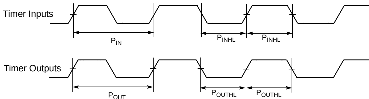
Figure 10-15 Timer Timing
