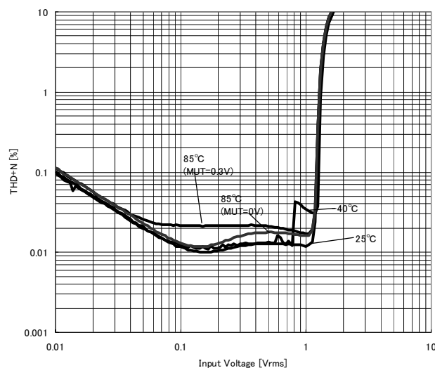
Mic AMP THD+N vs Input Voltage ( V_+ = 4.0\text{V} , MUT=0.3V, R_L = 5.1\text{k}\Omega , Gain=40dB, R_F = 300\text{k}\Omega , R_i = 3\text{k}\Omega , BW:400Hz~30kHz)
