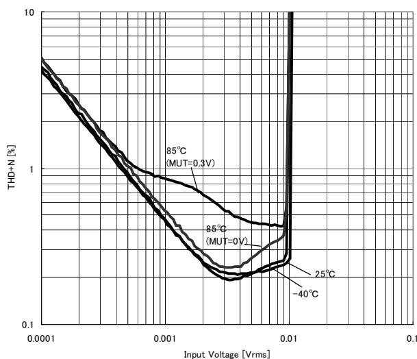
Mic AMP THD+N vs Input Voltage ( V_+ = 3.3\text{V} , MUT=0.3V, R_L = 5.1\text{k}\Omega , Gain=40dB, R_F = 300\text{k}\Omega , R_i = 3\text{k}\Omega , BW:400Hz~30kHz)
