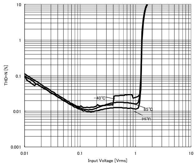
Mic AMP THD+N vs Input Voltage ( V_+ = 4.0\text{V} , MUT=0.3V, R_L = 5.1\text{k}\Omega , Gain=40dB, R_F = 300\text{k}\Omega , R_i = 3\text{k}\Omega , BW:400Hz~30kHz)
