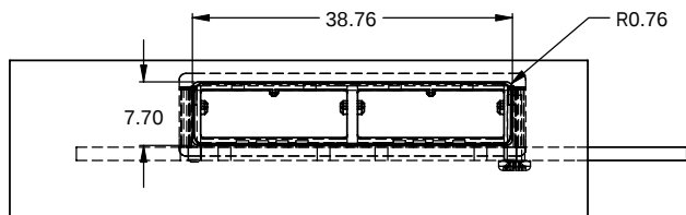
RECOMMENDED PANEL CUT-OUT
