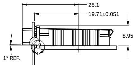
RECOMMENDED FACE PLATE TO LOCATING POST DISTANCE
