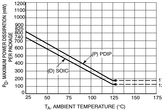
Figure 7. Ambient Temperature Power Derating
