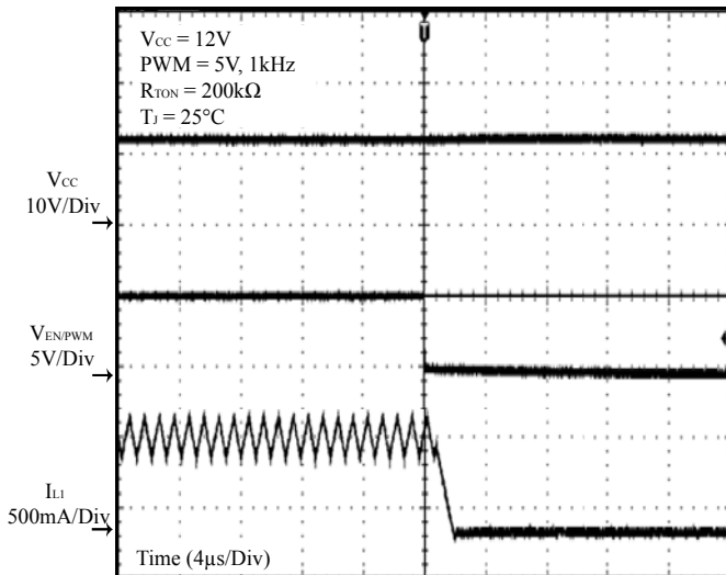
Figure 23 PWM Off
