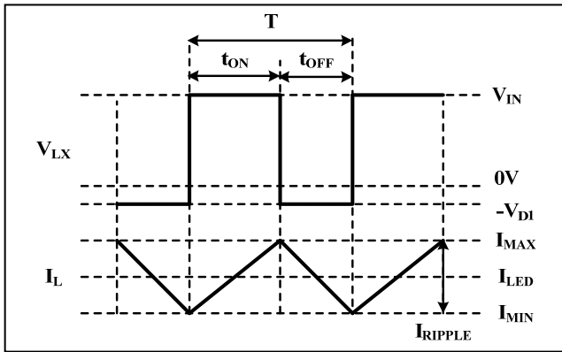
Figure 31 Operating Waveform
