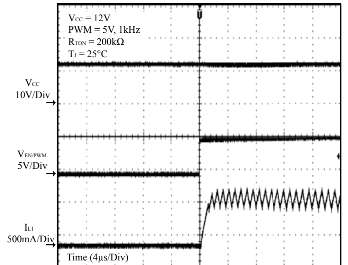
Figure 24 PWM On
