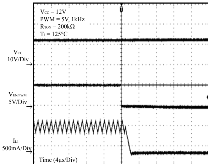
Figure 25 PWM Off
