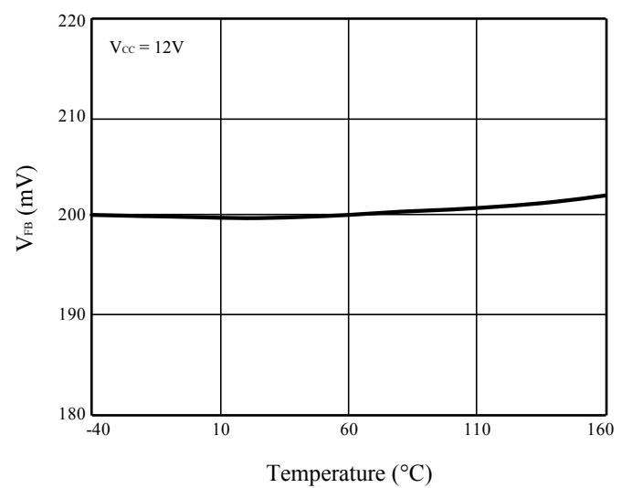
Figure 14 V_{FB} vs. Temperature
