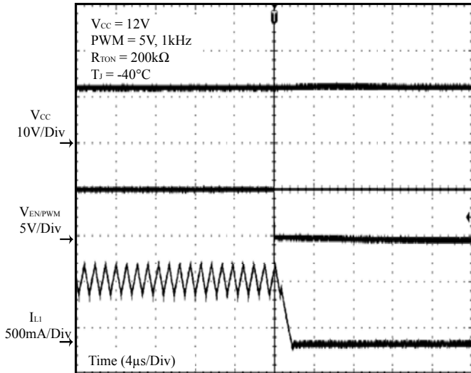
Figure 21 PWM Off
