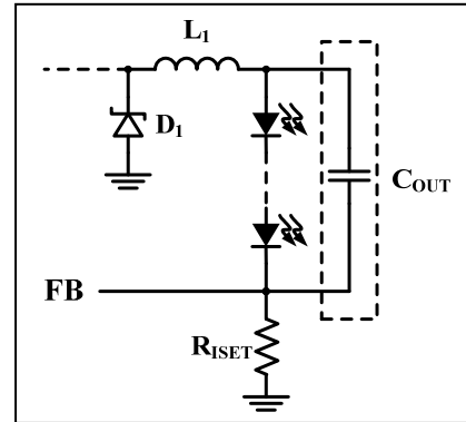
Figure 29 Adding Output Capacitor
