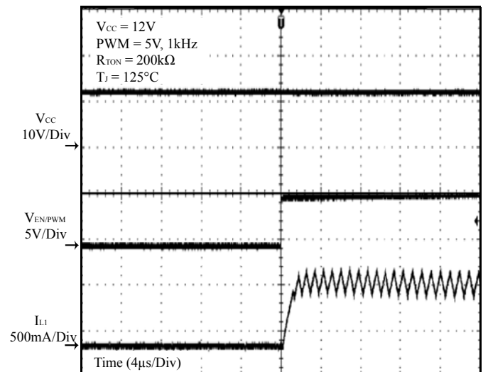
Figure 26 PWM On
