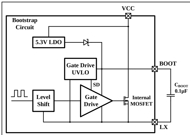
Figure 27 Bootstrap Circuit
