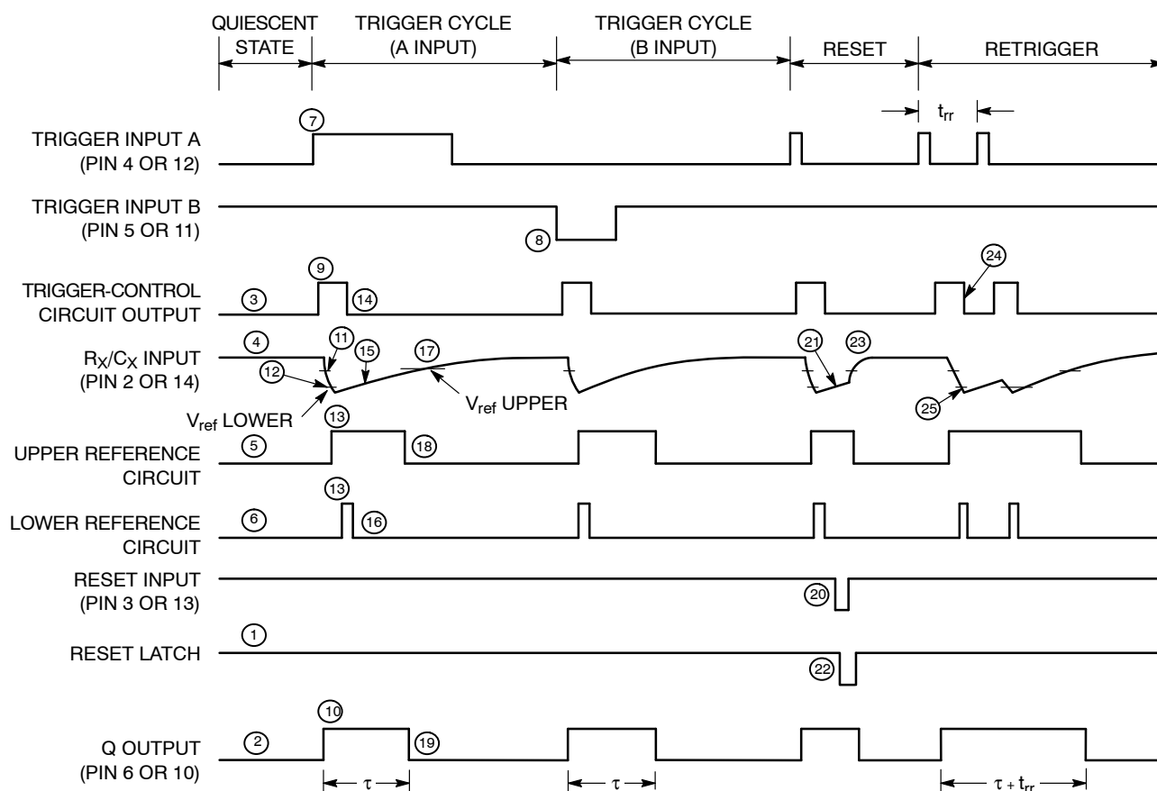
Figure 12. Timing Diagram
