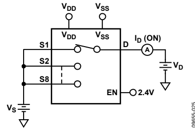
Figure 21. I_D (On)
