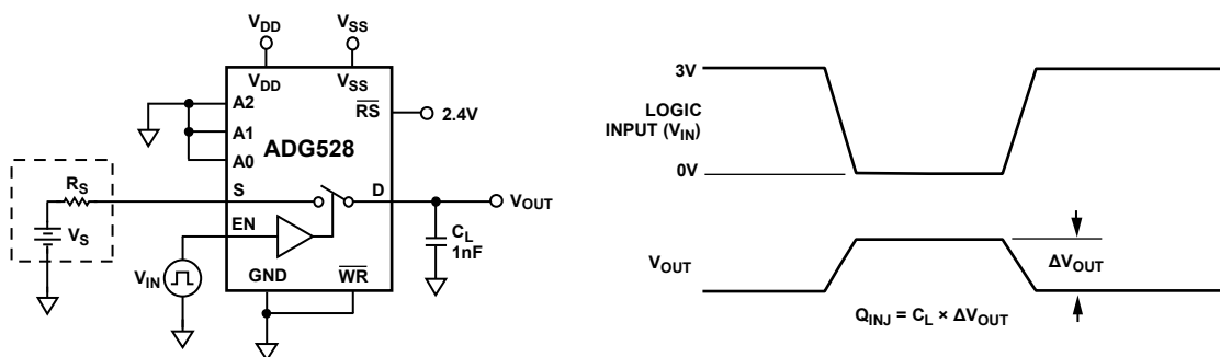
Figure 29. Charge Injection
