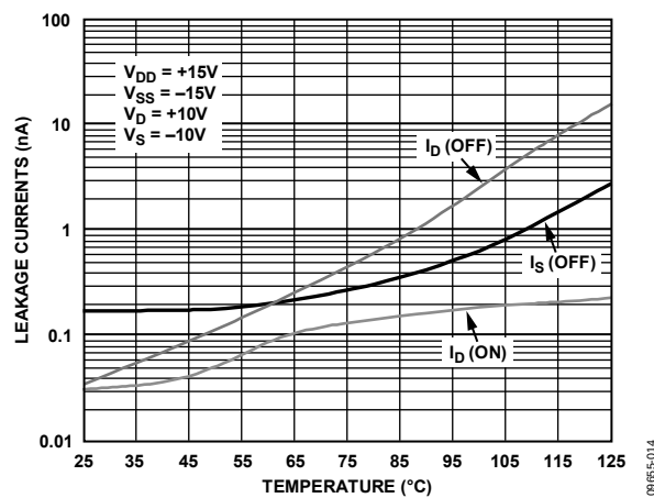
Figure 11. Leakage Currents as a Function of Temperature
