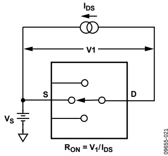
Figure 18. On Resistance
