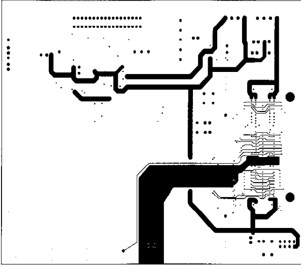
Figure 25. Power Plane 1
