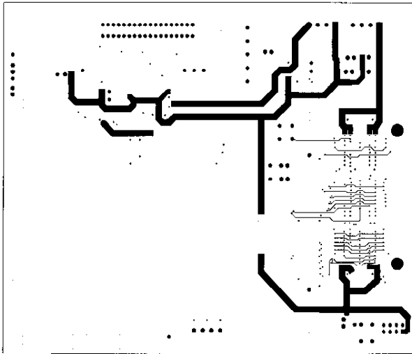
Figure 26. Power Plane 2
