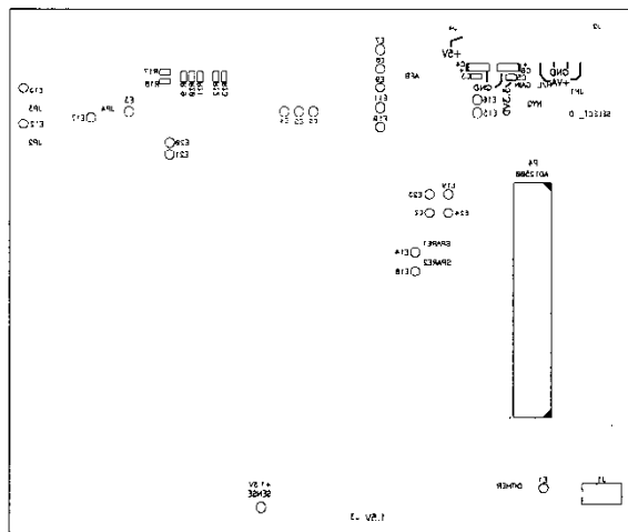
Figure 33. Bottom Silkscreen
