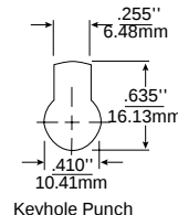
Keyhole Punch
