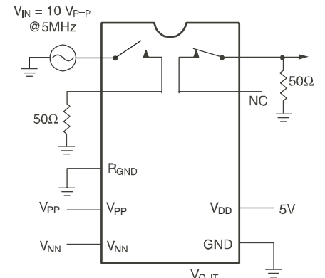
K_{CR} = 20 \log \frac{V_{OUT}}{V_{IN}} Crosstalk
