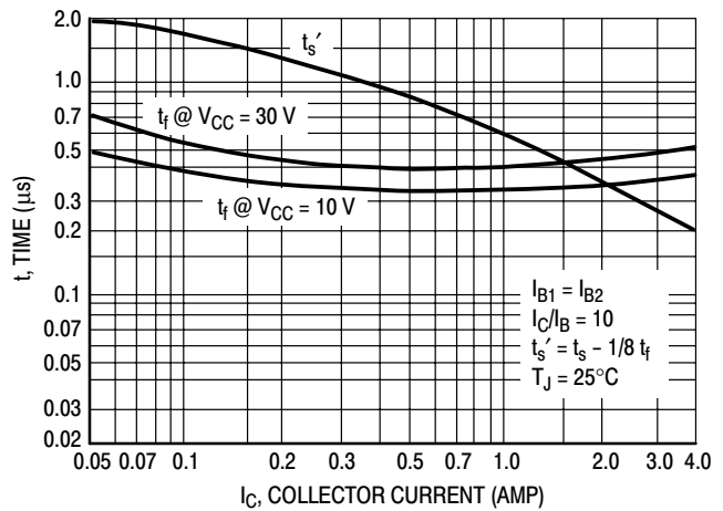
Figure 10. Turn-Off Time
