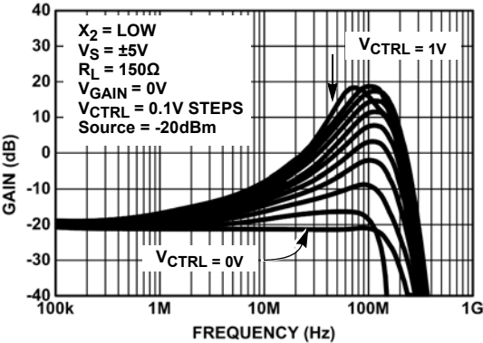
FIGURE 3. GAIN vs FREQUENCY FOR VARIOUS V CTRL
