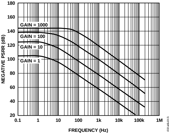
Figure 14. Negative PSRR vs. Frequency, RTI ( G = 1 to 1000)
