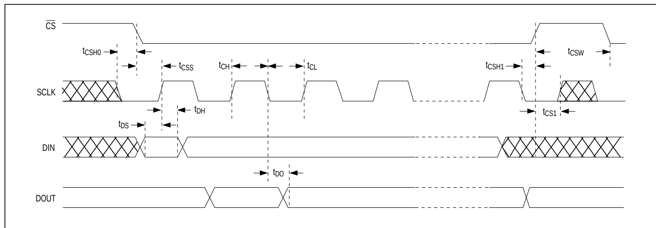
Figure 1. Timing Diagram
