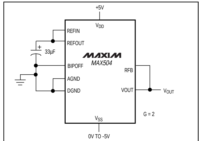
Figure 7. Unipolar Configuration (0V to +4.096V Output)
