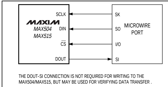
Figure 4. Microwire Connection
