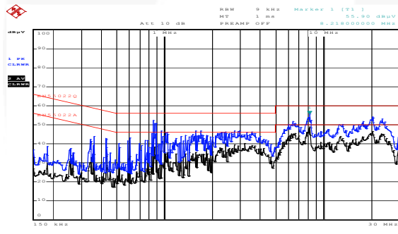
Figure 60. Line: 230 V AC / 50 Hz & 12 V O
