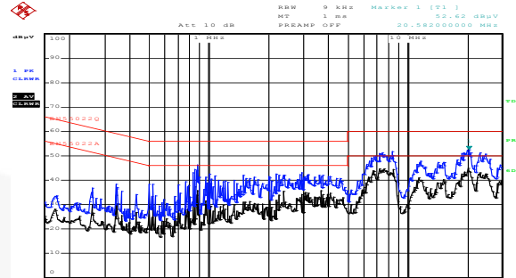
Figure 57. Neutral: 230 V AC / 50 Hz & 9 V O
