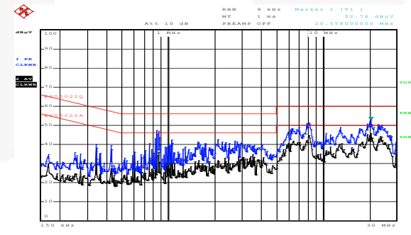
Figure 61. Neutral: 230 V AC / 50 Hz & 12 V O
