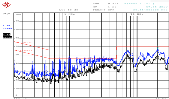
Figure 56. Line: 230 V AC / 50 Hz & 9 V O
