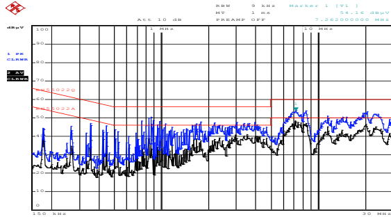
Figure 56. Line: 230 V AC / 50 Hz & 9 V O
