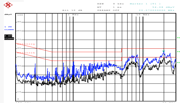
Figure 57. Neutral: 230 V AC / 50 Hz & 9 V O
