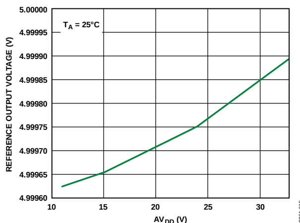
Figure 63. REFOUT Voltage vs. AV_{DD}
