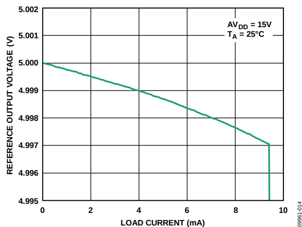
Figure 62. REFOUT Voltage vs. Load Current
