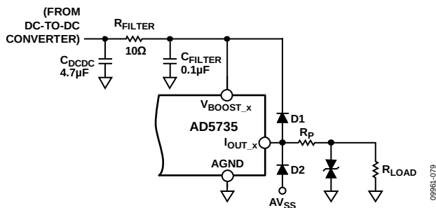
Figure 83. Output Transient Voltage Protection
