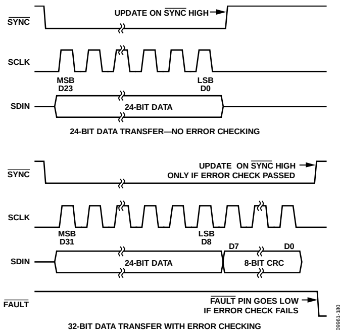
Figure 76. PEC Timing
