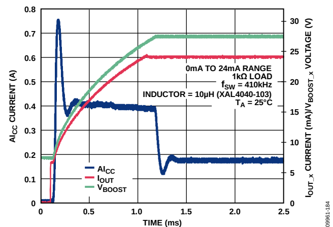
Figure 79. AI_{CC} Current vs. Time for 24 mA Step Through 1 k \Omega Load with Internal Compensation Resistor
