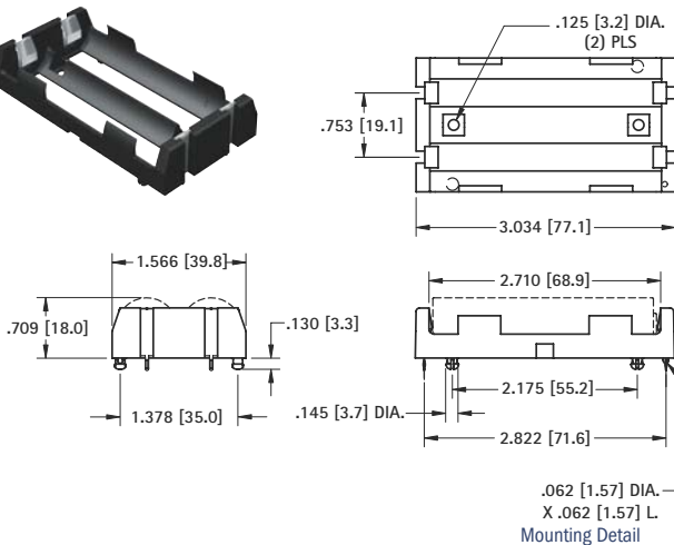
Mounting Detail
