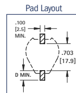
Surface Mount
