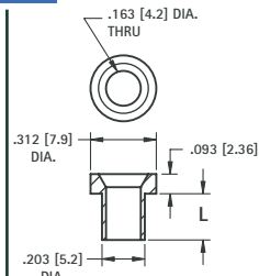
Accepts .175 (4.5) Plug
