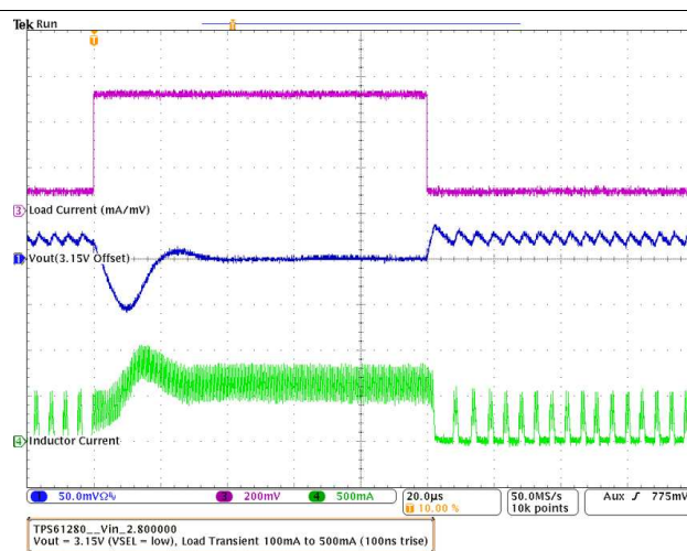
Figure 44. TPS61280, 81A Load Transient Response In PFM/PWM Operation
