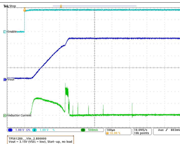
Figure 46. Start-Up at No Load
