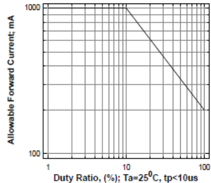
Allowable Forward Current Vs Duty Ratio
