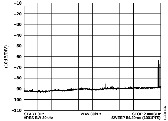
Figure 26. Single Tone SFDR f_{\text{DAC}} = 1966.08 \text{ MHz} , 4x Interpolation, f_{\text{OUT}} = 10 \text{ MHz} , -14 \text{ dBFS}
