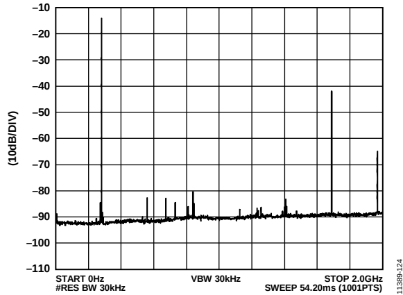
Figure 24. Single Tone f_{\text{DAC}} = 1966.08 \text{ MHz} , f_{\text{OUT}} = 280 \text{ MHz} , -14 \text{ dBFS}
