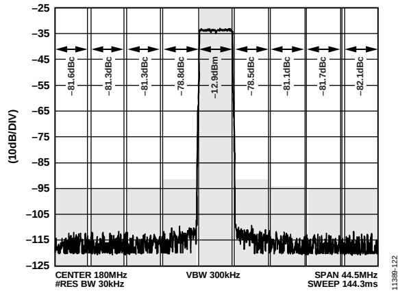
Figure 22. 1C 5 MHz BW LTE ACLR Performance, f_{\text{IF}} = 180 \text{ MHz} , f_{\text{DAC}} = 1966.08 \text{ MHz}
