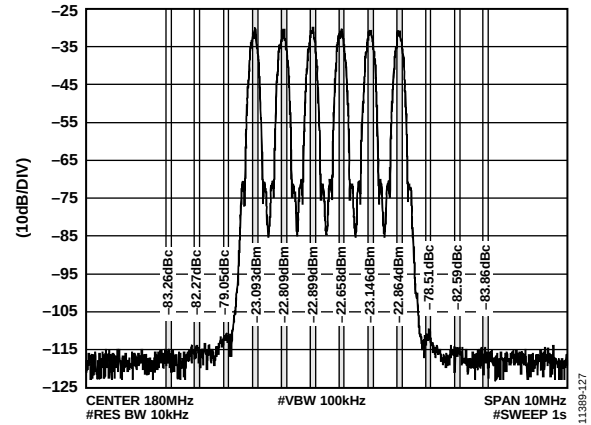
Figure 27. 6-Channel (6C) Spaced by 600 kHz GSM, Enhanced Data Rates for GSM Evolution (EDGE) Adjacent Channel Power (ACP) IMD Performance, f_{\text{IF}} = 180 \text{ MHz} , f_{\text{DAC}} = 1966.08 \text{ MHz}
