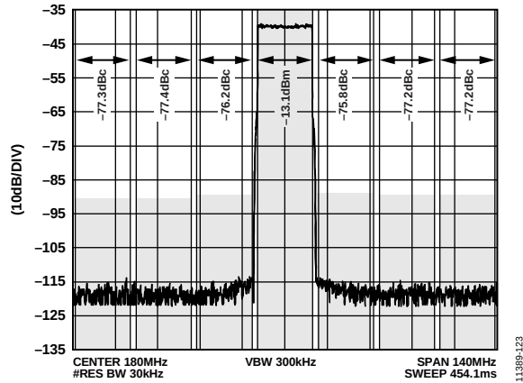
Figure 23. 1C 20 MHz BW LTE ACLR Performance, f_{\text{IF}} = 180 \text{ MHz} , f_{\text{DAC}} = 1966.08 \text{ MHz}
