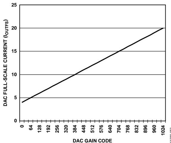
Figure 80. DAC Full-Scale Current ( I_{OUTFS} ) vs. DAC Gain Code
