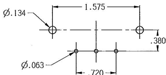
PCB MOUNTING
