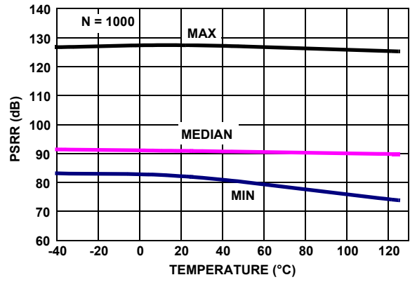
FIGURE 26. EL8173 PSRR vs TEMPERATURE, V_+, V_- = \pm 1.2V \text{ TO } \pm 2.5V
