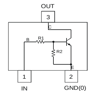
Schematic and Pin Configuration
