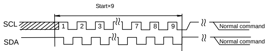
Figure 37-(c) START × 9 + command input * Start command from START input.
