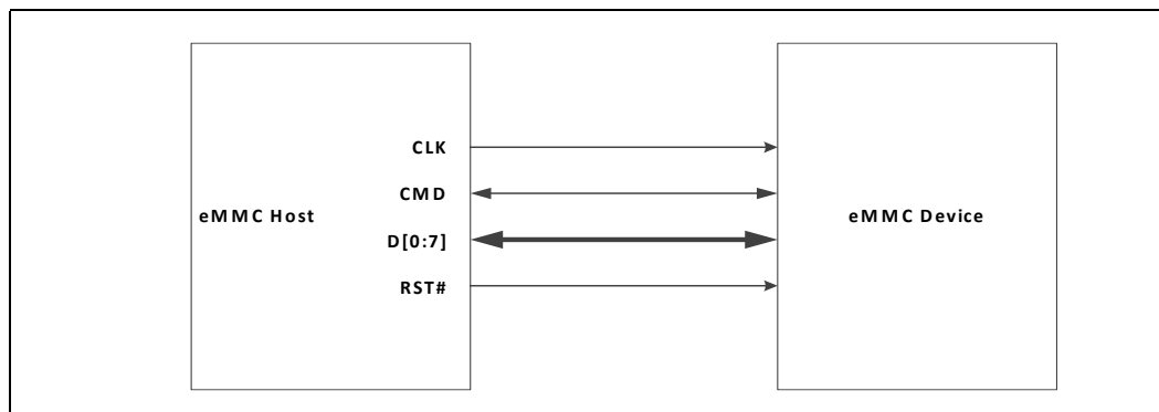
Figure 100.eMMC Interface
