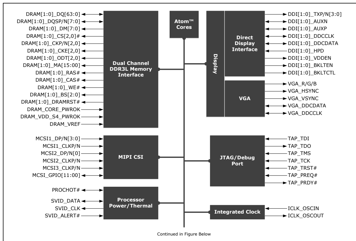
Figure 2. Signals (1 of 2)
