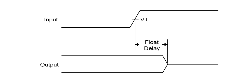
Figure 85. Pulse Width
