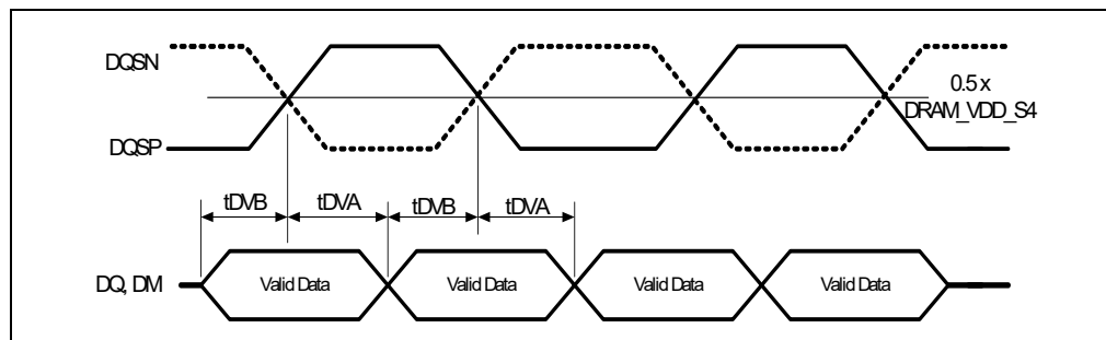
Figure 21. DDR3L Write Pre-ample Duration
