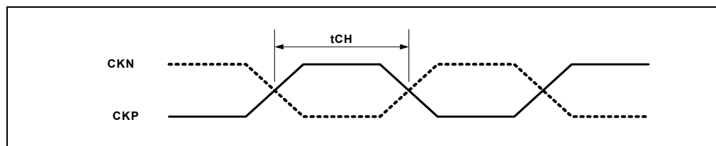
Figure 30. DDR3L CK Low Time
