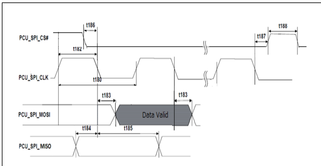
Figure 67. SPI NOR Timing
