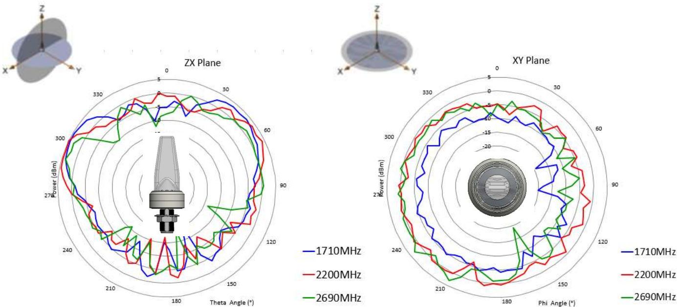
Elevation Plane
