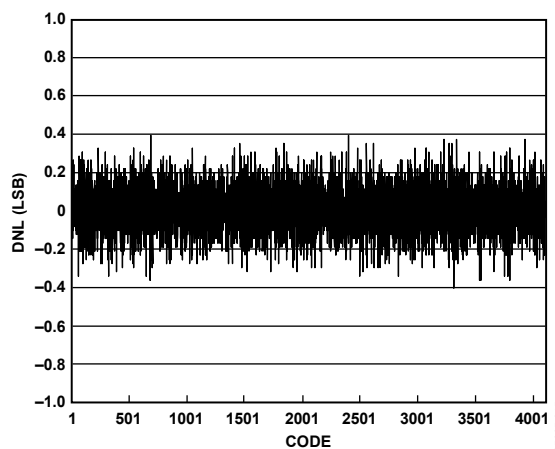
Figure 15. ADC DNL
