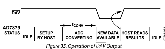
Figure 35. Operation of \overline{\text{DAV}} Output
