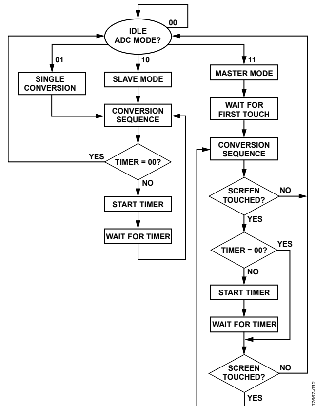
Figure 32. Conversion Modes
